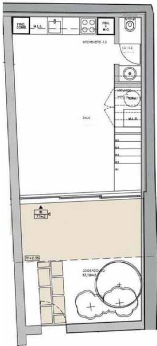
Planta Piso Inferior | Lower Floor Plant
